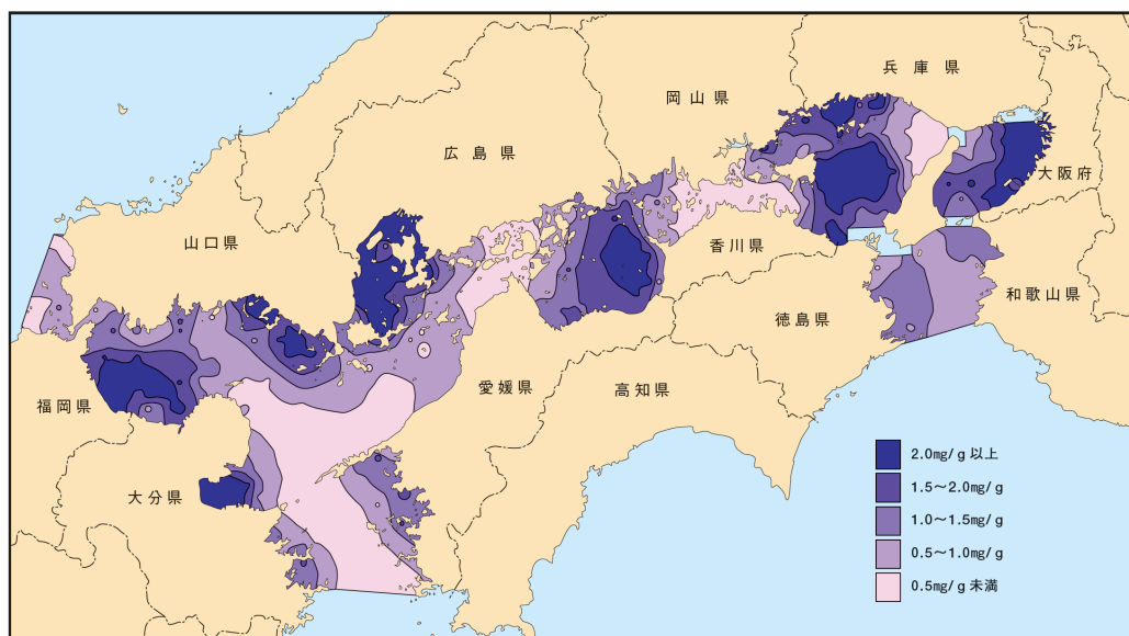
[全窒素]
